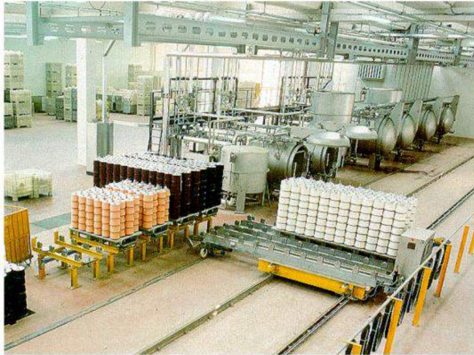
Photo: RBNO robot package dyeing plant
