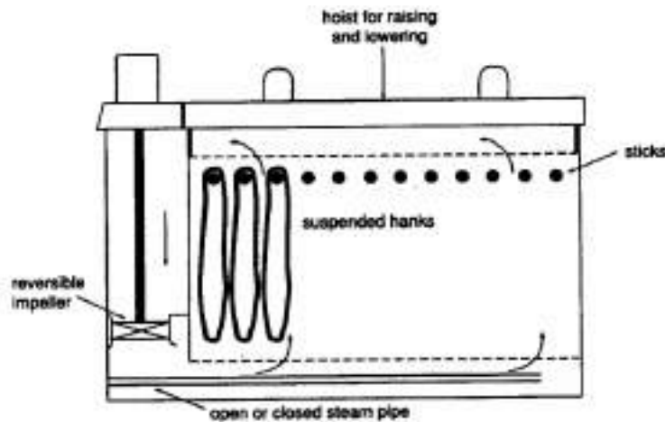
Figure: Hank dyeing machine.
